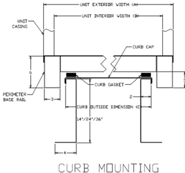
Figure 16: Roof Curb Mounting Detail
